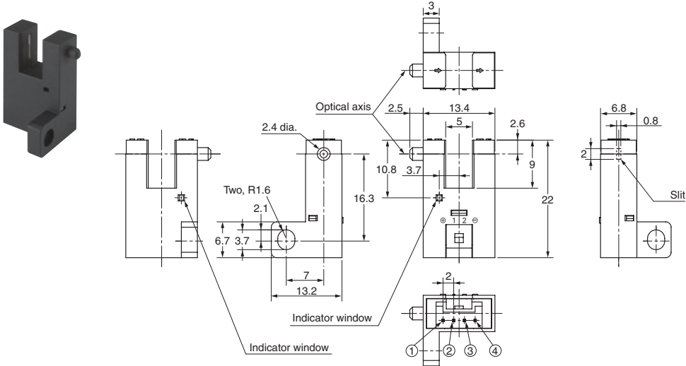
Mounting screw holes
