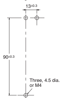
Mounting Holes
